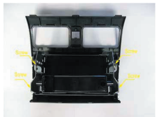
Remove complete panel. Remove 4 screws en disable metal bracket. Place back panel and connect all wiring.
