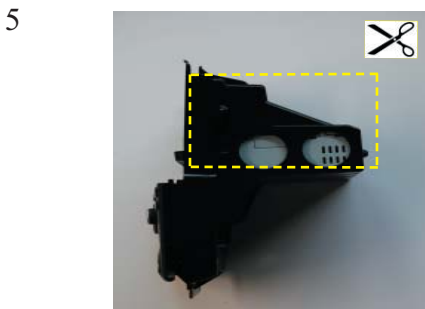
Remove the plastic at the backside of the panel.
