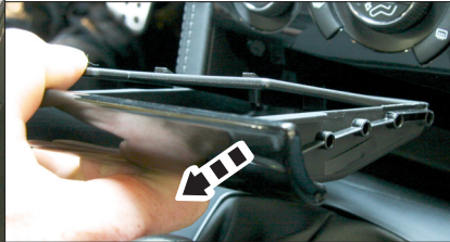
1. Remove lower tray under OEM head unit
