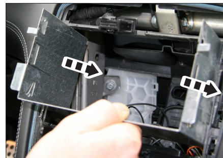
8. Mount metal frame to dash board
