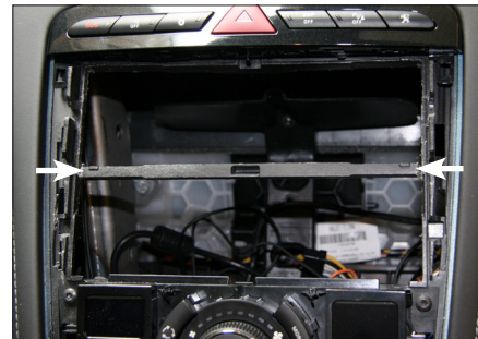
6. Cut away middle bar to clear space for double DIN head unit
