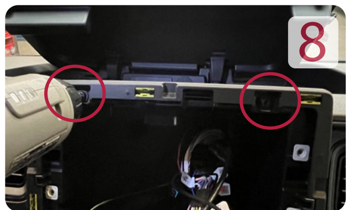
Install the 2 screws at the top of the frame
