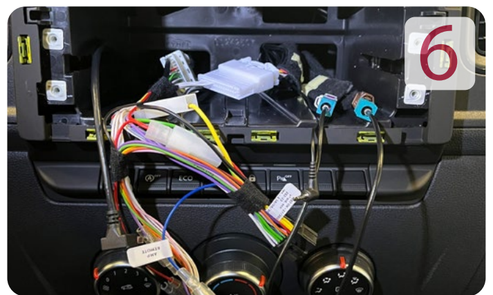
Connect the cables as shown in the picture. DAB, FM and Microphone on the left / Remaining connectors on the right.
