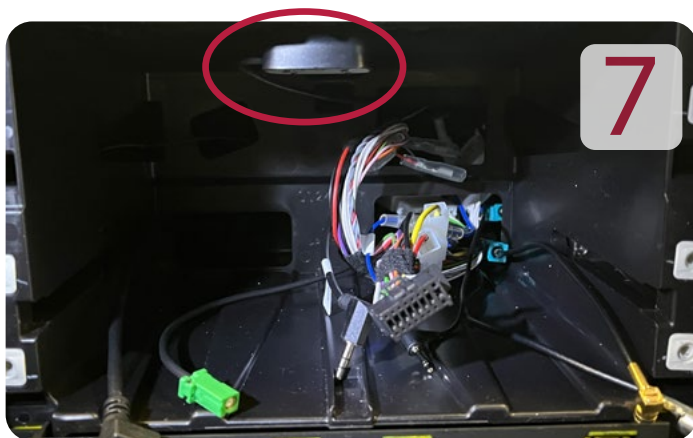
Tuck the harnesses and interface box as shown, to make it easier to install the car radio. To save time, the GPS antenna can be glued in place as shown in the picture (NOTE: the glue has to be very strong and the antenna's head should be facing upwards).
