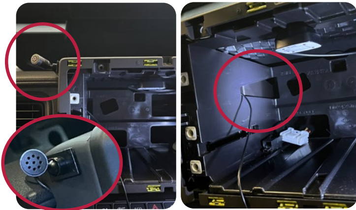
Suggested position for the microphone: top left side of the original frame.
