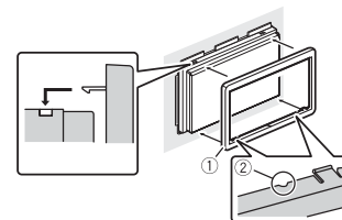
1 Trim ring
