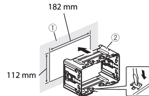
1 Dashboard 2 Holder
