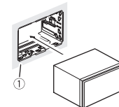
1 Dashboard
